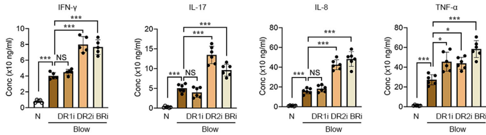
FIGURE 4. Measurement of inflammatory cytokine levels in DE-induced LGs using ELISA. IFN- \gamma , IL-17, IL-8, and TNF- \alpha expression levels in LGs were measured 14 days after DE induction with or without dopamine receptor inhibitors. BRI, both receptors inhibited; DR1i, SCH-23390; DR2i, melperone; N, naive condition. All experiments were repeated three times in at least triplicate ( n = 5 , one-way ANOVA and Bonferroni-corrected Dunnett test for post hoc analysis). * P < 0.05 . ** P < 0.01 . *** P < 0.001 . NS, not significant.
