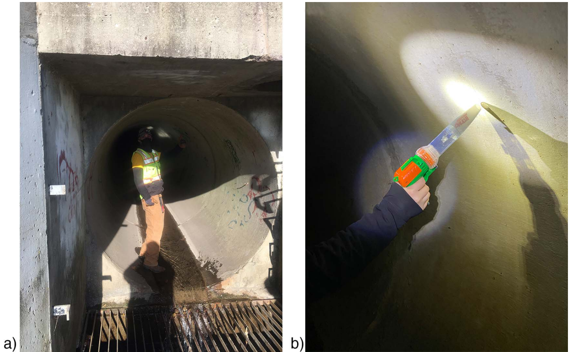
Fig. 1. (a) Inspector standing within the outfall of one of the examined belowground stormwater pipes; (b) inspector collecting adult Culex off a wall approximately 0.25 mi (400 m) into pipe.
