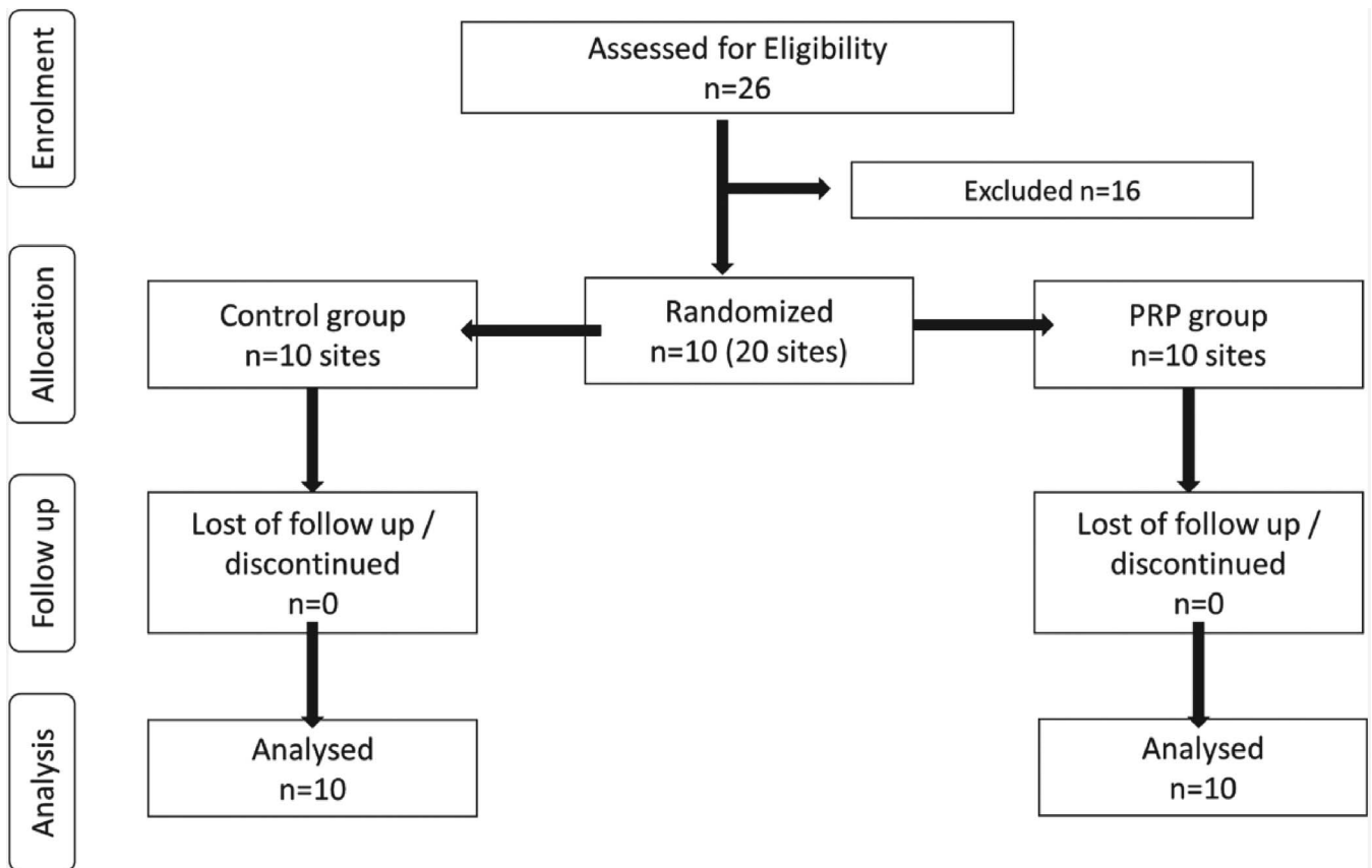
Figure 2. CONSORT flowchart.
