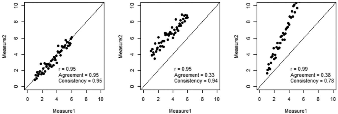
Figure 2. Three scenarios of rater reliability. In the left plot, the two measurements have a relationship of Y = X + \epsilon , where \epsilon is the random error. In the middle plot, the relationship is Y = X + 3 + \epsilon . In the right plot, the relationship is Y = 2X + \epsilon .
