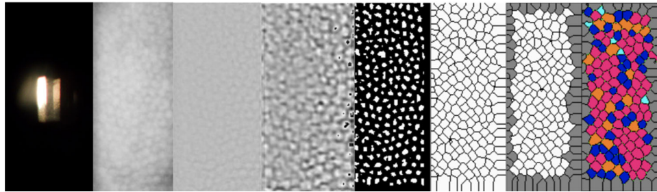
Figure 4. Image analysis processing pipeline. Left to Right: Raw Image, Cropped Image, Light Normalization, Smoothing, KH Algorithm, Thinning, Artifact Removal, and Triple-Point Analysis.
