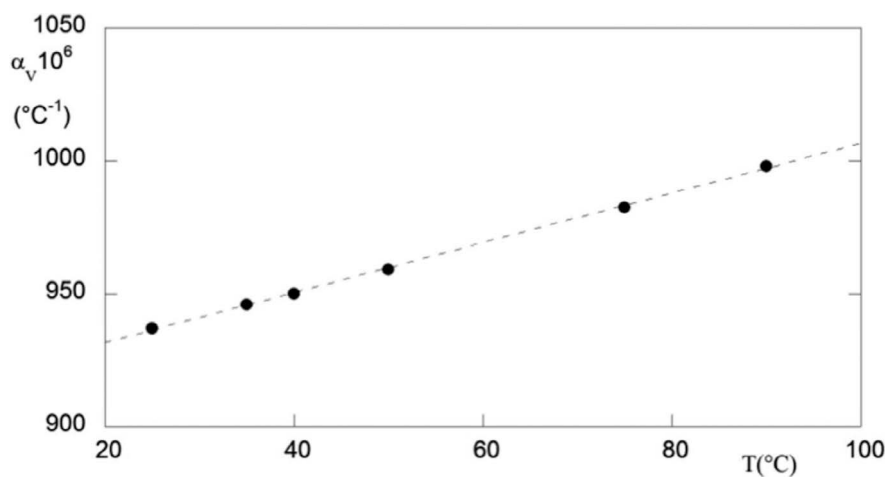
Figure 4. Thermal expansion versus temperature for silicone oil. The curve was evaluated directly from experimental volumetric data.
