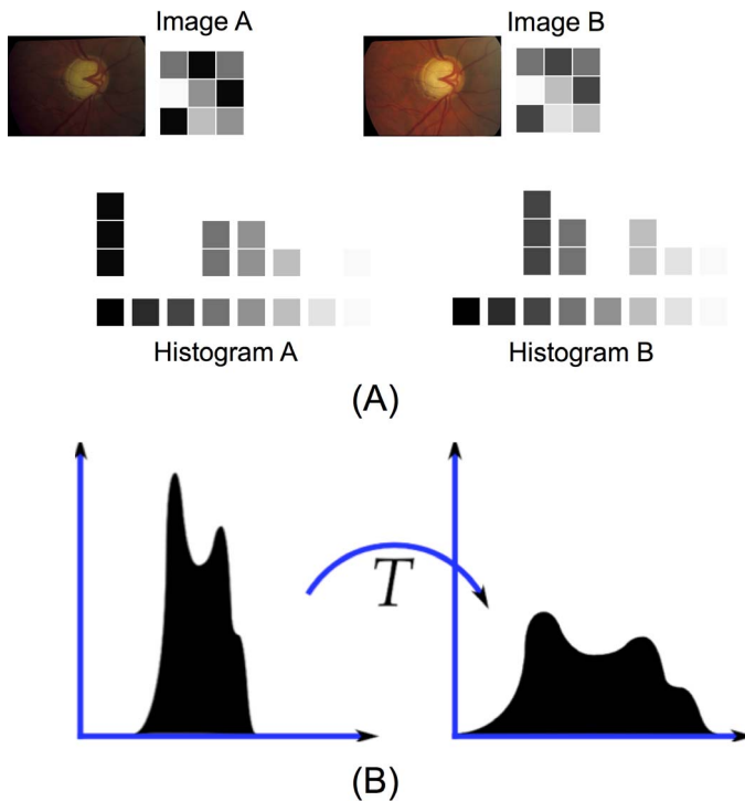
Figure 1. (A) Image A and image B differ in their global illumination. However, their histograms have similar patterns. The histograms are for demonstration purposes only. (B) Histogram matching is a process in which an image is modified such that its histogram matches that of another. Histogram equalization is a special case in which the specified histogram is uniformly distributed and, as such, the transformed histogram becomes flatter.
