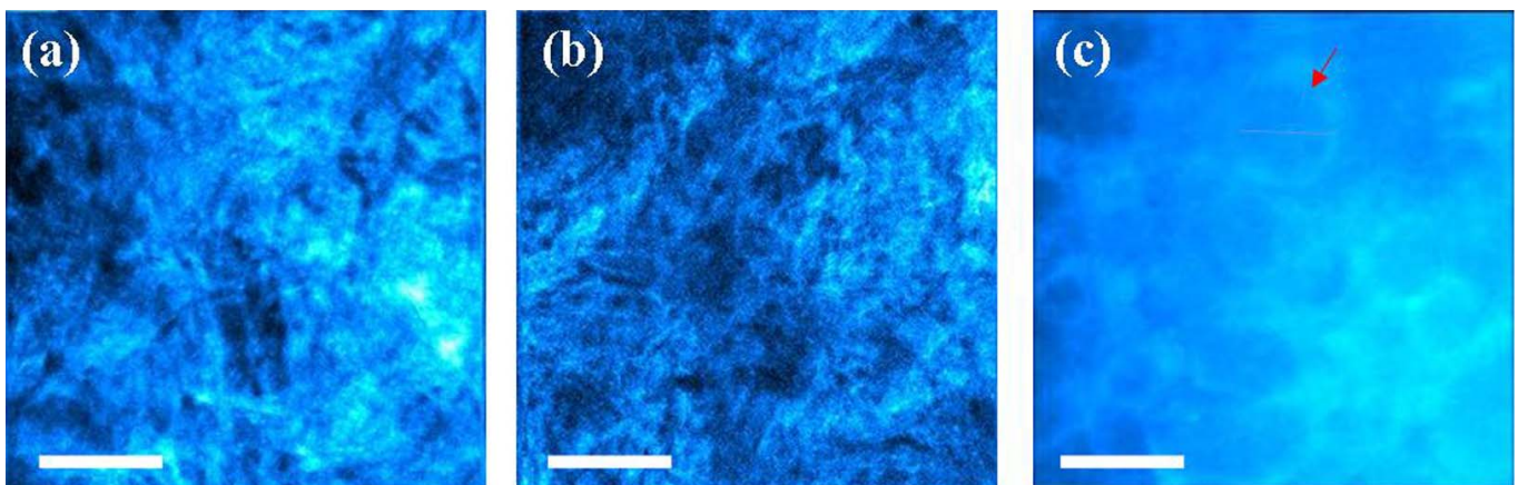
Figure 3. SHG images of ex vivo pathological corneas (depth location: 50\ \mu\text{m} ): keratoconus (a, b) and bullous keratopathy (c). Scale bar: 50\ \mu\text{m} .
