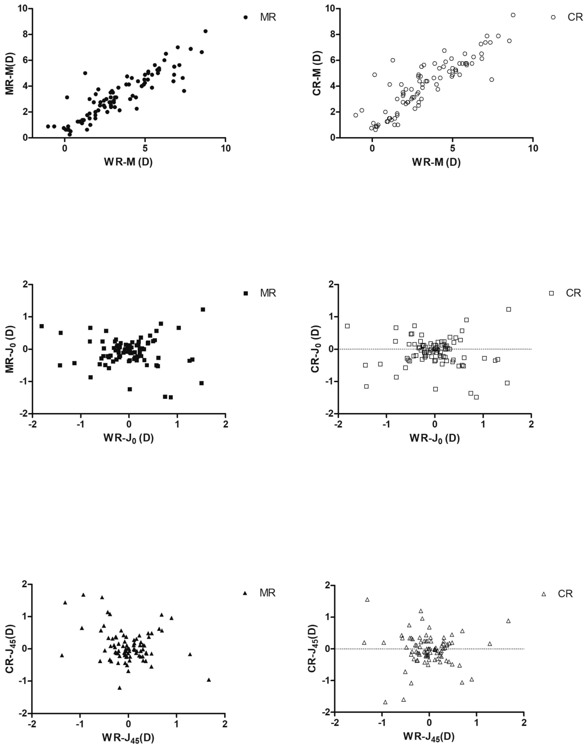
Figure 1. Scatter plot of vector components between WR and CR/MR. WR, wavefront supported custom ablation refractive; D, diopter.
