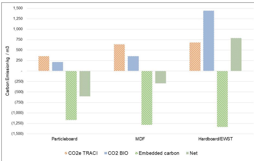
Figure 1.—Carbon emissions for CO_{2e\ TRACI} and CO_{2\ BIO} , embedded carbon (flow), and net CO_2 expressed in kg of CO_2 for particleboard, medium density fiberboard (MDF), and hardboard–engineered siding and trim (EWST) based on 2019 North American shipments only.
