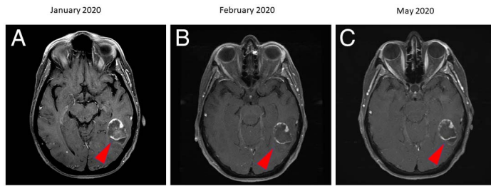
Figure 1. (A) The T1 post-contrast magnetic resonance image of the brain in a 42-year-old woman with metastatic hormone-positive breast cancer in January 2020 showed a 3.8 \times 2.9 -cm well-demarcated lesion involving the posterior medial and inferior temporal gyri with a 1.1 \times 0.9 -cm enhancing nodule. (B) Repeat imaging in February 2020 showed a minimal decrease in lesion size, which then measured 3.7 \times 2.8 cm. (C) Additional imaging performed in May 2020 showed the 3.7-cm previous cystic left temporal lesion unchanged, but with the development of eight new supratentorial metastases measuring up to 4 mm.
