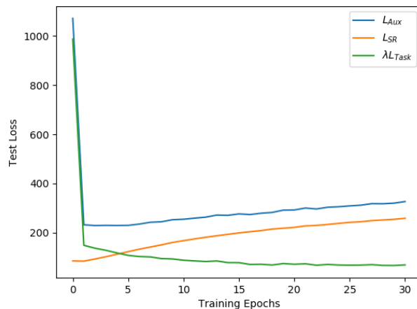
Figure 8: Training an auxiliary quine with Adamax
