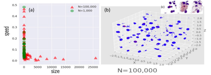
Figure 2: (a) Speed and size distribution of clusters for N = 1,000 and 100,000. (b) Clusters positions in 3D space and (c) an explosion of a cluster for N = 100,000 .
