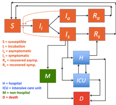
Figure 1: Flow diagram of the SEIRS based model system. As only ~3% are vaccinated by March 5, 2021 they are not explicitly modeled.
