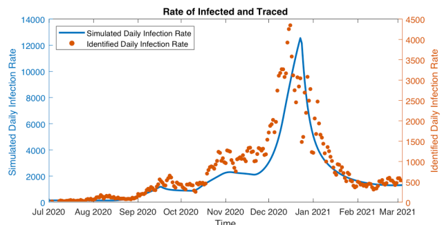
Figure 4: Time evolution of simulated rate of new infected I_{inf} (solid blue) and daily reported infection tracing [11] rate (red dots). Note different scales. See text for details.
