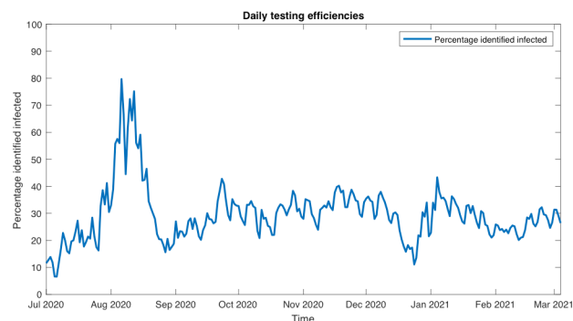
Figure 5: Efficiency of daily infection tracing in Denmark Jul. 1, 2020 – Mar. 5, 2021 expressed as DT^{avg}(t) . See text for details.
