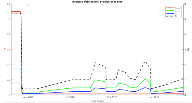
Figure 2: \beta and \mathcal{R}_0 profiles. Initial free pandemic is followed by an initial effective lockdown of Mar. 11, 2020. Slow controlled reopenings in late spring and early summer are followed by opening of bars and nightlife by mid-August. A second boost occurs mid fall and infections continue to increase due to winter and Christmas followed by a 2 nd full lockdown by Dec. 25. The steady increase thereafter is due to the increasing B117 mutant and slow reopening late Feb. 2021.
