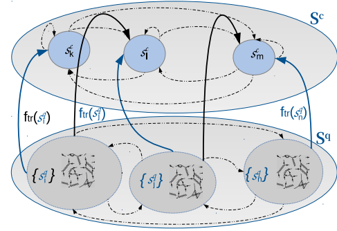
Figure 2: Schematic view of a general hierarchical system under investigation. Quantum dynamics described by S^q is observed at the classical level and described by S^c .
