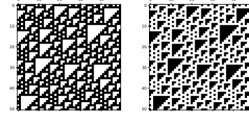
Figure 1: Space-time diagram of ECA rule 110 on the left and its dual rule 137 on the right.
