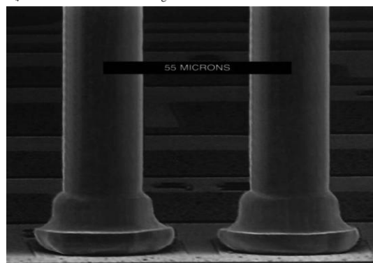
Figure 3: Scanning electron photomicrograph of ultrafine pitch (55μm) thermo-sonic ball bonding. The bonds were made on a K&S Model 8020 automatic ball bonder using 23μm (0.9 mil) diameter gold alloy wire. Pad metallization was Al + 1% Si + 2% Cu on SiO 2 with nominal 1μm thickness. (Photomicrograph courtesy of L. Levine, K&S).
