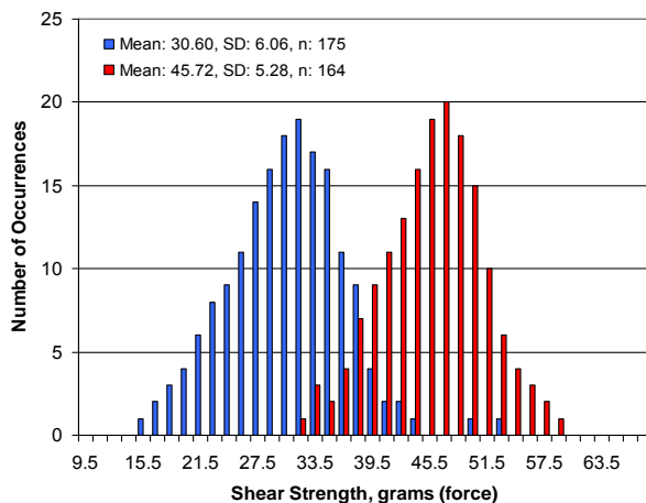
Figure 2: Histograms of gold thermo-sonic ball bond shear strengths for bonds placed on aluminum metallization (over silicon). Histogram A (left or blue bars) are the shear test results after the bonding machine was set up using the wire-bond pull test. Histogram B (right or red bars) are the shear test results after the bonding machine was optimized using the ball shear test.
