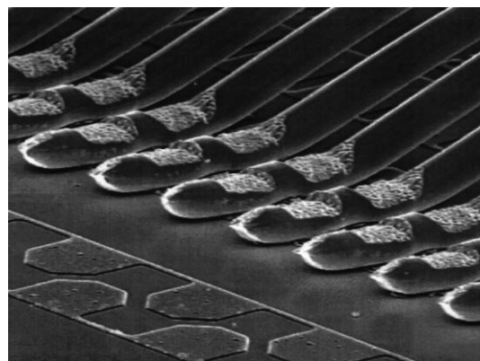
Figure 4: Scanning electron photomicrograph of ultrafine pitch (40μm) wedge bonds. The bonds were made on a K&S Model 8060 automatic wedge bonder using 20μm (0.8 mil) diameter gold alloy wire. Pad metallization was Al + 1% Si + 2% Cu on SiO 2 with nominal 1μm thickness. (Photomicrograph courtesy of L. Levine, K&S).
