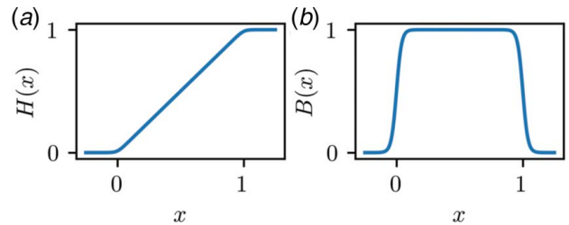
Fig. 3 (a) Smooth approximated fixbound function H(x) which models the piecewise function in Eq. (9). (b) Boxcar function B(x) which allows for an analytical conditional reassignment. Both functions are plotted with a stiffness parameter of k = 50 .
