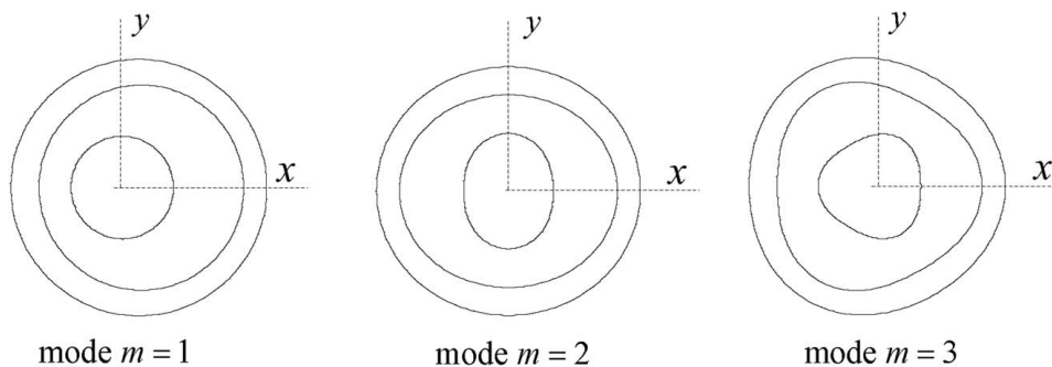
Fig. 3 The plane strain bifurcation modes for m = 1, 2, 3
