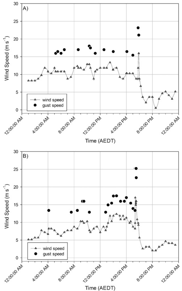
FIG. 2. Wind speeds and wind gusts for (a) Melbourne International Airport and (b) Avalon Airport on 21 Nov 2016. Thunderstorm activity occurred between 1700 and 1800 AEDT.
