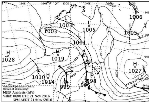
FIG. 1. Weather map for Australia at 0600 UTC (1700 AEDT) 21 Nov 2016.
