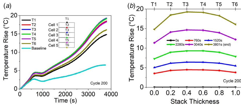
Fig. 3 (a) Representative temperature rise during discharge of baseline cell and five-cell stack in cycle 200 and (b) representative spatial distribution of temperatures inside the five-cell stack at different stage of discharge in cycle 200
