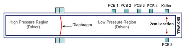
Fig. 1 Schematic of the shock tube facility indicating positions of pressure transducers and test section location
