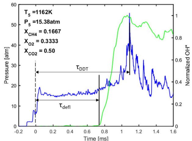
Fig. 3 Typical experimental pressure and emission traces with labeled definitions of ignition for the 50% CO 2 -diluted mixture
