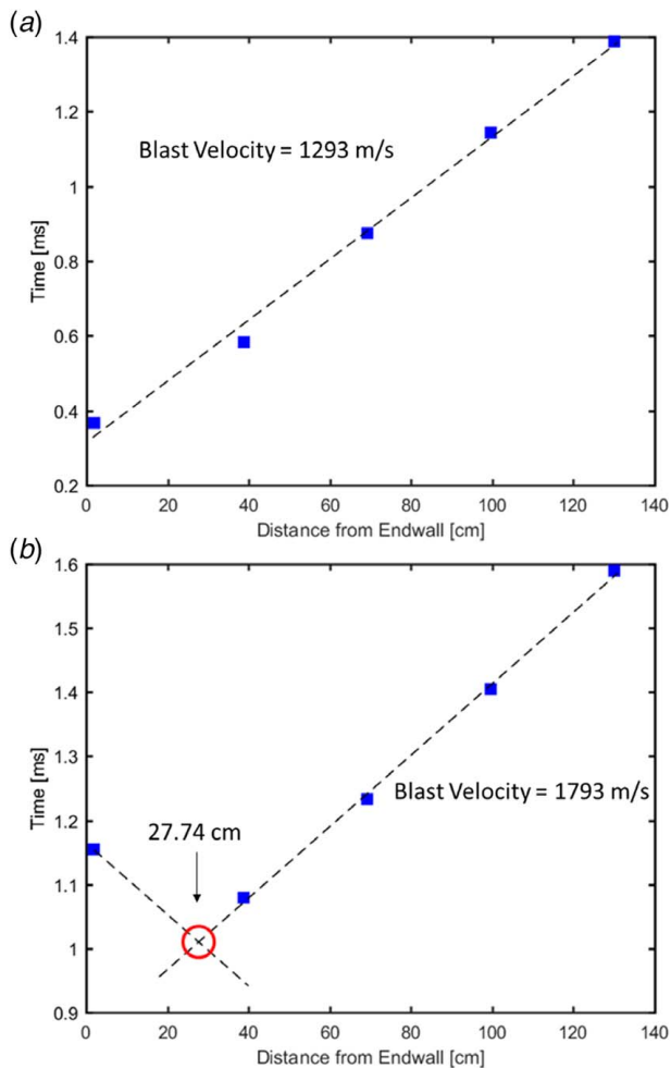
Fig. 6 Experimental detonation maps for (a) a homogeneous ignition event from the CO 2 -diluted mixture and (b) an inhomogeneous ignition event from the N 2 -diluted mixture; blast location is marked by an open red circle. Blast velocities and location are shown.
