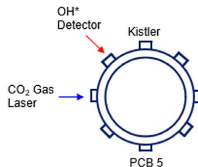
Fig. 2 Schematic showing circumferential positions of various diagnostics used (note this is in plane at the 2-cm location)
