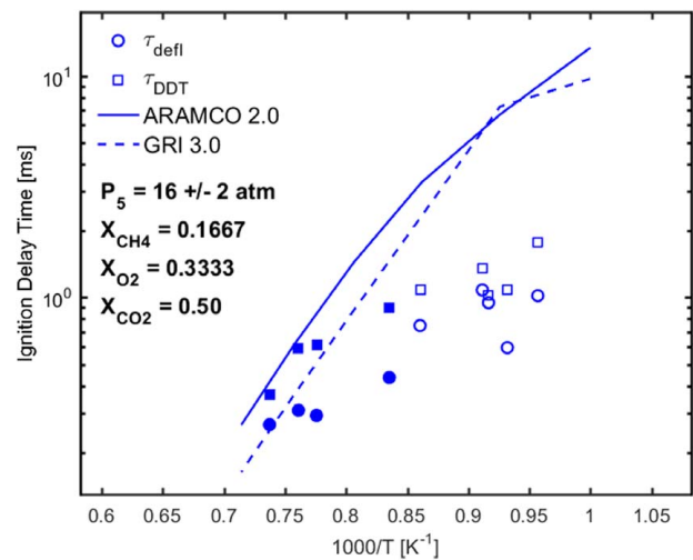
Fig. 7 Experimental definitions of ignition delay times compared to model predictions using chemkin-pro of the CO 2 -diluted mixture. Homogeneous events are indicated with filled markers.
