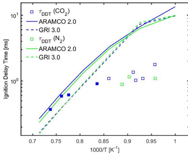
Fig. 9 Experimental ignition delay times based on immense pressure rise associated with detonation arrival compared to model predictions using chemkin-pro. Both \text{CH}_4/\text{O}_2/\text{CO}_2 and \text{CH}_4/\text{O}_2/\text{N}_2 mixture data are presented.
