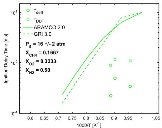
Fig. 8 Experimental definitions of ignition delay times compared to model predictions using chemkin-pro of the N 2 -diluted mixture. Inhomogeneous events are indicated with open circles and squares.
