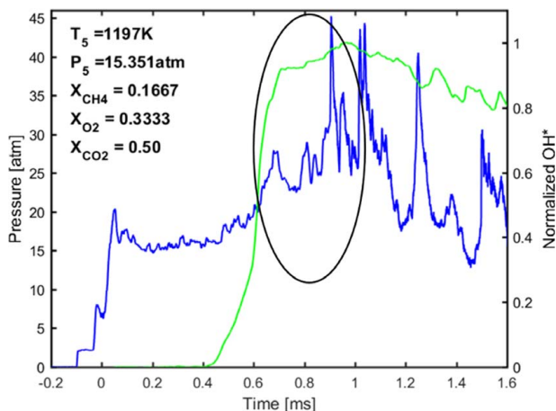
Fig. 4 Pressure and emission traces for the 50% CO 2 -diluted mixture shown with a circled region of ignition
