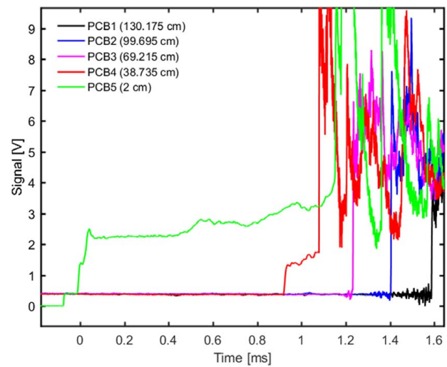
Fig. 5 Pressure traces measured via PCBs showing arrival of detonation with noted location from the end wall
