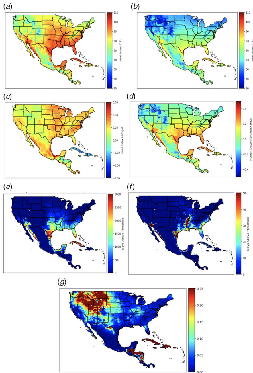
Fig. 2 Climatology of (a) maximum summer mean HI 1990–2019, (b) minimum summer mean HI, 1990–2019, (c) summer HI trend, 1990–2019 (°F/year), (d) mean summer HDI, 1990–2019, (e) summer days between 90^{\circ}\text{F} \leq \text{HI} \leq 102^{\circ}\text{F} , 1990–2019, (f) summer days \text{HI} \geq 102^{\circ}\text{F} , 1990–2019, and (g) summer HI trend p -value, 1990–2019. Climatology, grid averages, and grid trends were computed using 3-h NCEP–NARR data during a 30-year period (1990–2019).
