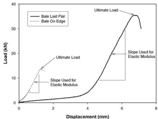
FIGURE 13. Averaged load-displacement responses for plastered straw bales.
