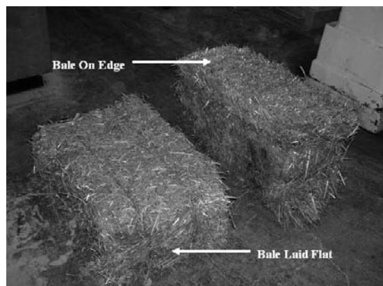
FIGURE 2. Bales laid flat and on edge.
