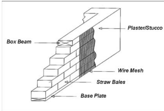
FIGURE 1. Simplified typical wall details.
