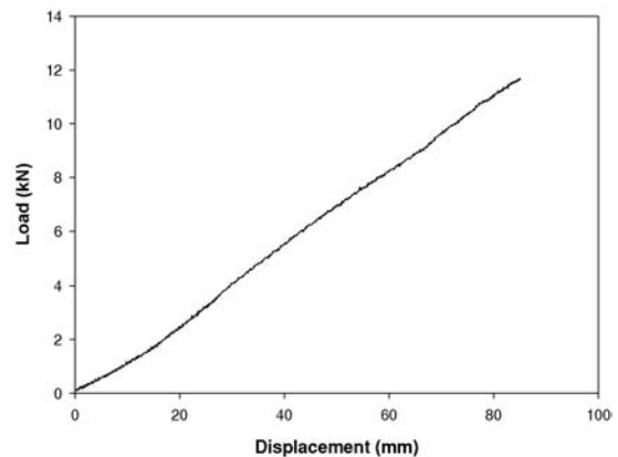
FIGURE 8. Load-displacement response for on-edge, un-plastered straw bale.
