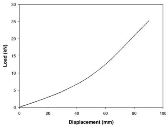
FIGURE 7. Load-displacement response of flat, un-plastered straw bale.
