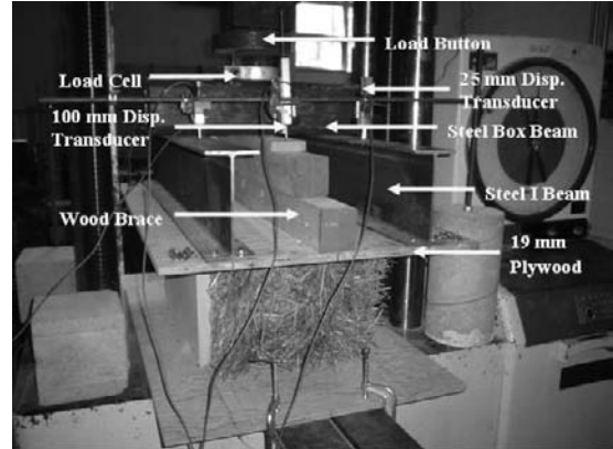
FIGURE 5. Loading apparatus.
