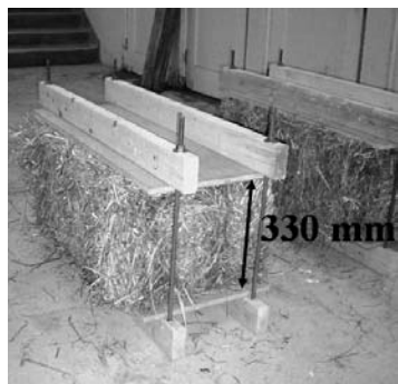
(a) Bale compressed in jig.
