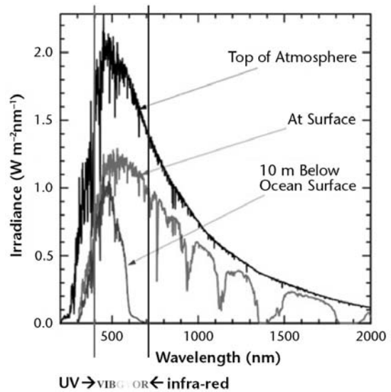
FIGURE 2. Solar and visible spectrum.
