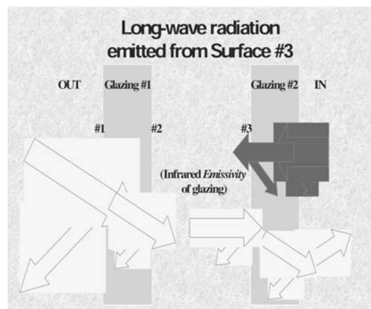
FIGURE 7. Radiant transfer in inner glazing (#2).
