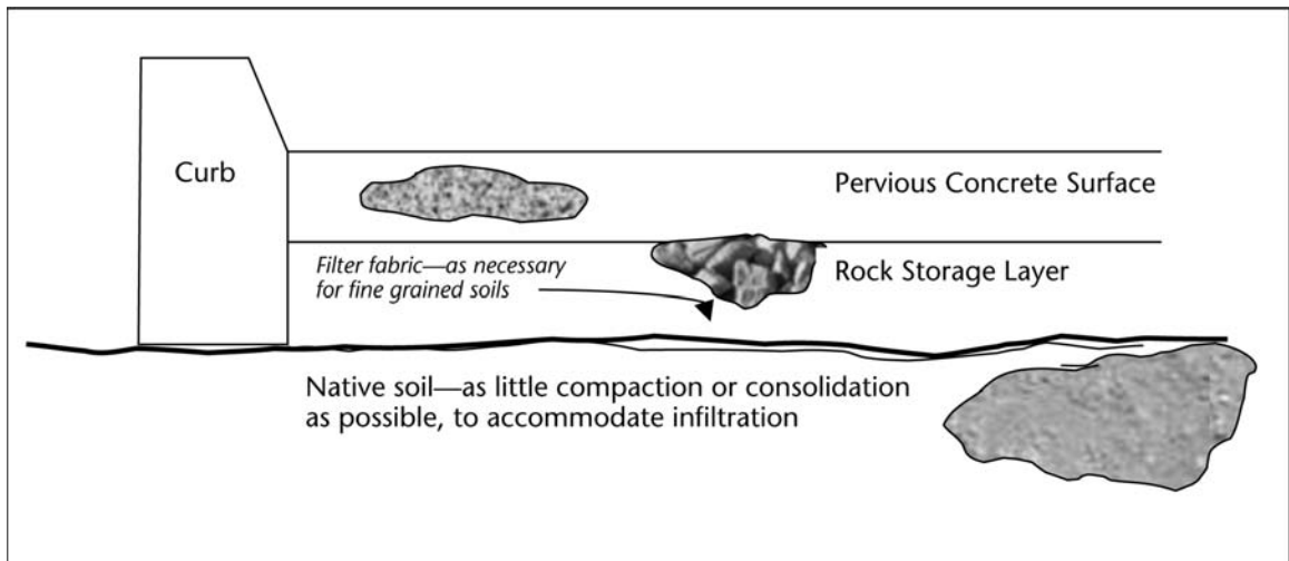
FIGURE 4. Sketch of typical pervious pavement/sidewalk installation.
