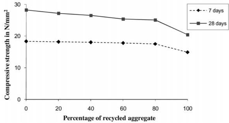
FIGURE 3. Effect of RA Content on Compressive Strength.
