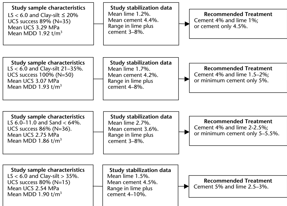
FIGURE 2. Stabilizer treatment summaries and recommendations for the four categories of soils deemed favorable for stabilization. UCS success is the percentage of samples with UCS \geq 2 MPa as tested in the study.
