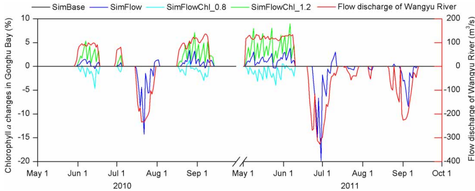
Figure 7 | The change in average chlorophyll a in Gonghu Bay due to water transfers to the Wangyu River during the modeling period.
