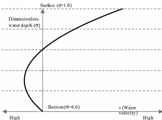
Figure 3 | Empirical parabola representing vertical profiles of the horizontal water velocity (redrawn from Huang et al. (2012a)).
