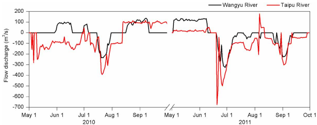
Figure 4 | The inflow and outflow discharges of the Wangyu and Taipu Rivers between May and September of 2010 and 2011. The positive and negative values represent inflow and outflow river, respectively.
