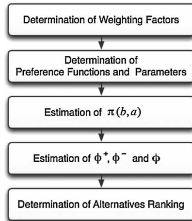
Figure 2 | Concept diagram of the PROMETHEE procedure.
