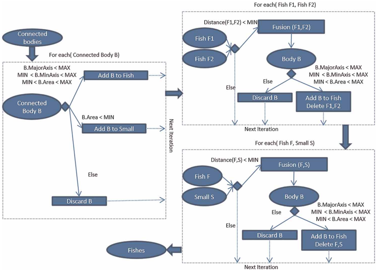
Figure 5 | Diagram of the algorithm used to interpret the segmented image.
