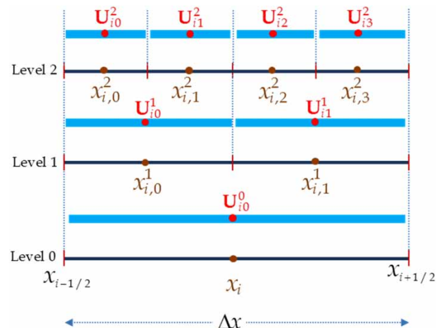
Figure 4 | Local multiresolution stencil \{I_{ij}^n\} embedded within cell i .
