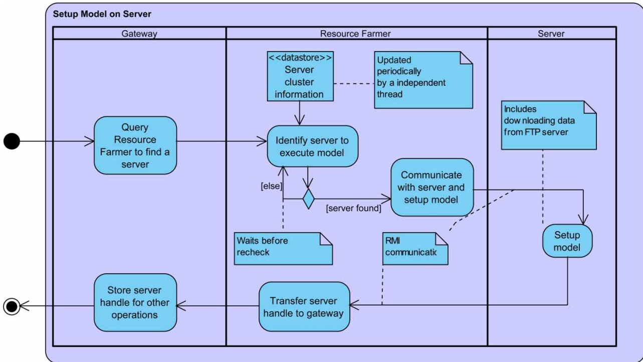
Figure 5 | Illustration of the 'Setup Model on Server' activity involving communication between the three components.
