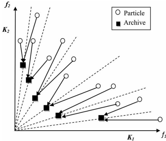
Figure 2 | Finding the best local guide for each particle of the population using Sigma method (Mostaghim & Teich 2003).
