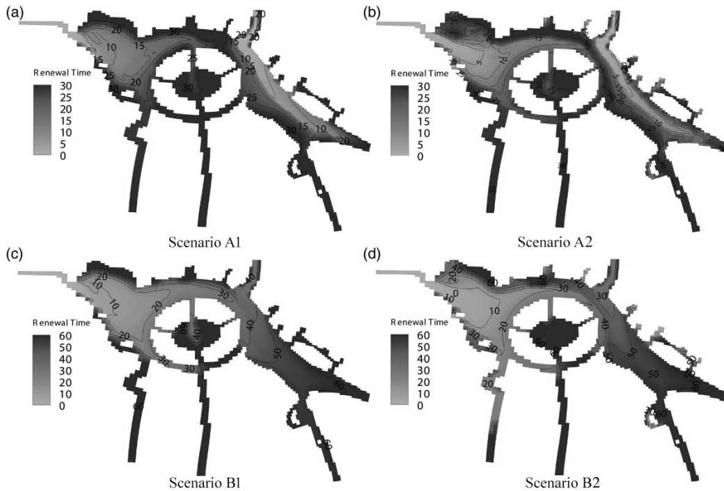
Figure 7 | Spatial distribution of the LRT within the lake for: (a) A1, 10 \text{ m}^3/\text{s} , 30 days; (b) A2, 10 \text{ m}^3/\text{s} , 30 days, plus pumped inflows at the bays and pumped outflow at the inner lake; (c) B1, 5 \text{ m}^3/\text{s} , 60 days; (d) B2, 5 \text{ m}^3/\text{s} , 60 days, plus pumped inflows at the bays and pumped outflow at the inner lake.
