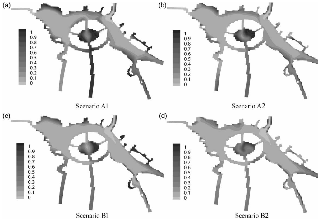
Figure 6 | Renewal pathways (vertically averaged and plotted at the last day) for: (a) A1, 10 \text{ m}^3/\text{s} , 30 days; (b) A2, 10 \text{ m}^3/\text{s} , 30 days, plus pumped inflows at the bays and pumped outflow at the inner lake; (c) B1, 5 \text{ m}^3/\text{s} , 60 days; (d) B2, 5 \text{ m}^3/\text{s} , 60 days, plus pumped inflow at the bays and pumped outflow at the inner lake. Light colour represents 'freshwater' with a value of '0' indicating complete renewal.
