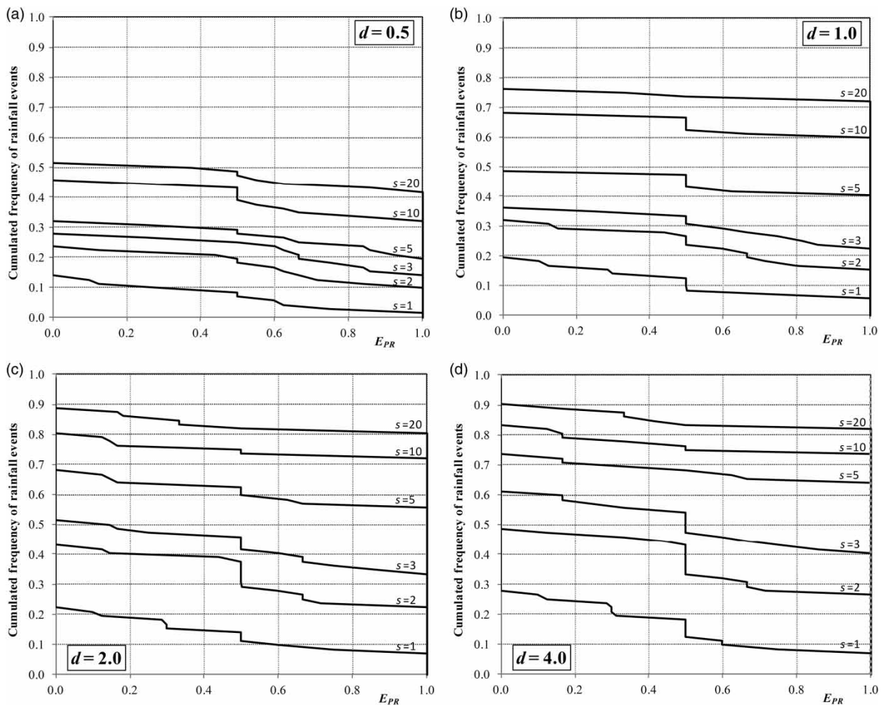
Figure 5 | Tank peak retention efficiency as a function of the cumulated relative frequency of rainfall events in the year. The household is assumed to host one person. (a) d = 0.5 ; (b) d = 1.0 ; (c) d = 2.0 ; (d) d = 4.0 .
