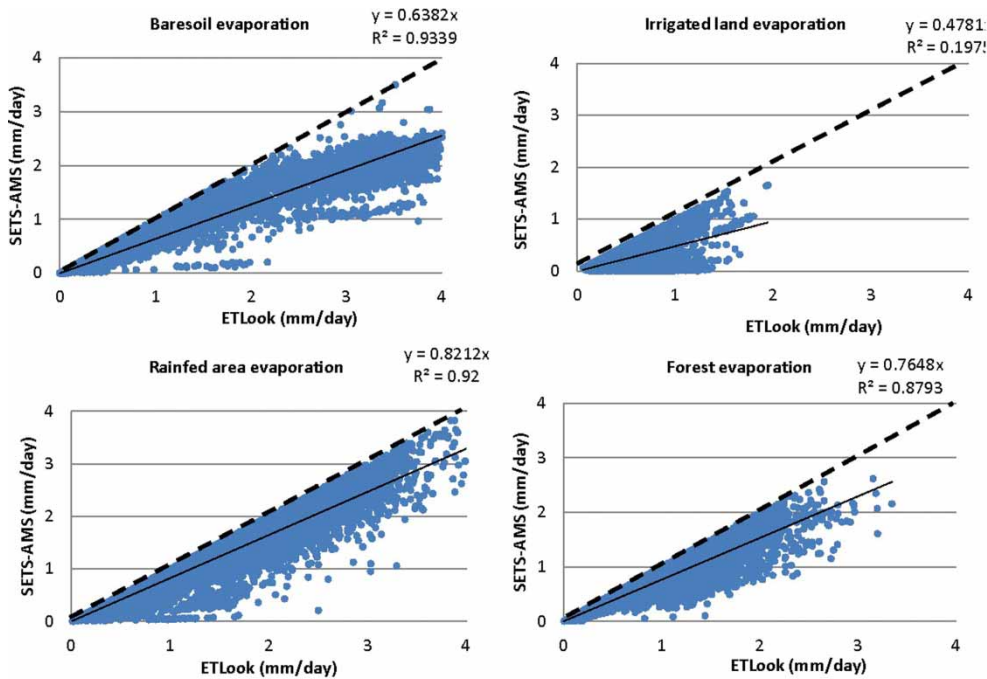
Figure 4 | Comparison between E (mm/day) estimates of SETS-AMS and ETLook for different land cover types.
