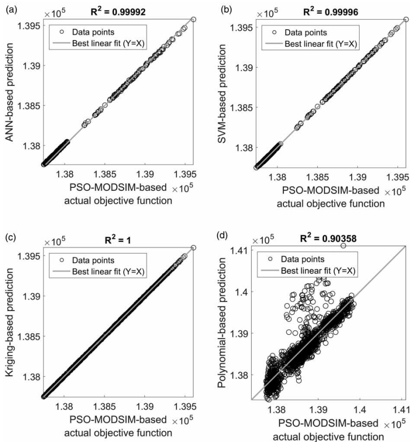
Figure 9 | (a) ANN, (b) SVM, (c) kriging, (d) polynomial-based predictions at the last iteration of the ASSF approach (y-axis) vs. PSO-MODSIM-based actual objective function values (x-axis).
