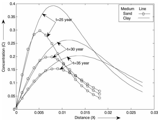
Figure 3 | Concentration distribution for the exponential decreasing form of unsteady form of velocity for time T > T_p with average porosity of the medium.
