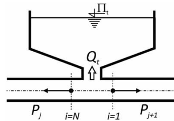
Figure 6 | Surge tank.
