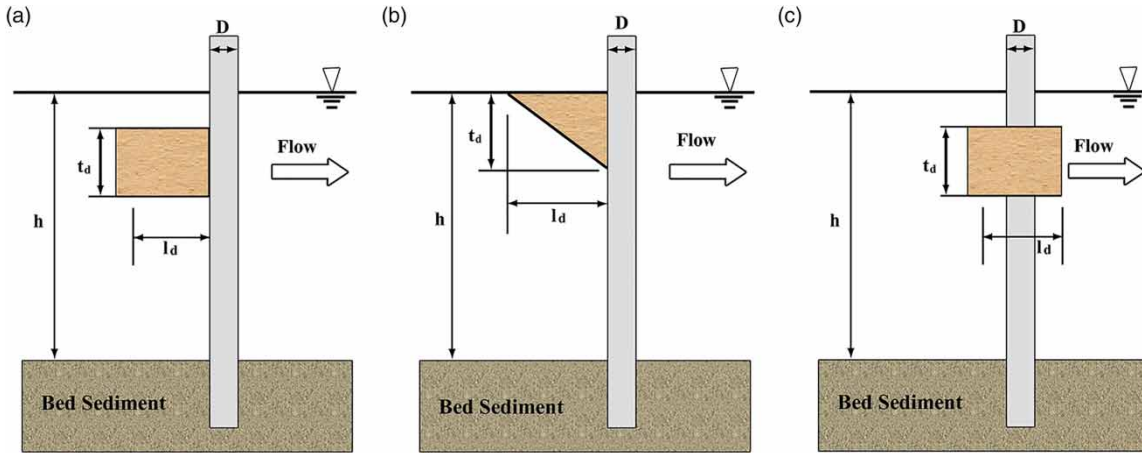
Figure 2 | Various configurations of debris accumulations used in the Melville & Dongol (1992), Pagliara & Carnacina (2011a), and Sok et al. (2015) experiments with: (a) rectangular; (b) triangular-conical; (c) circular geometries.
