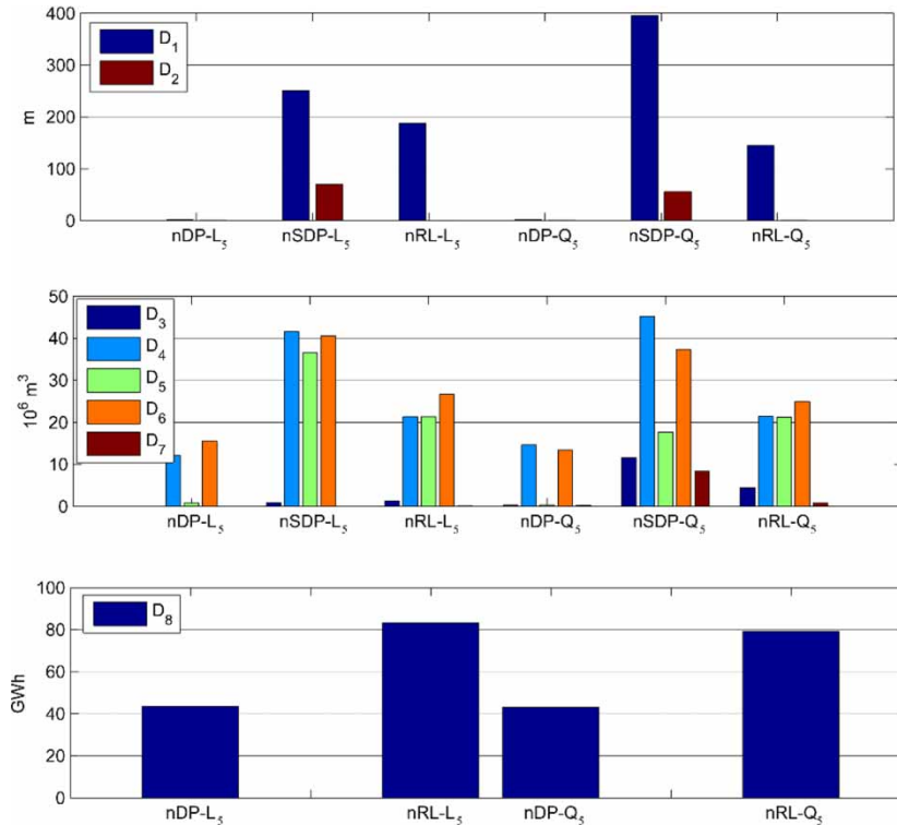
Figure 5 | nDP-L 5 , nDP-Q 5 , nSDP-L 5 , nSDP-Q 5 , nRL-L 5 and nRL-Q 5 comparison of the sum of minimum level ( D_1 ) and maximum level ( D_2 ) deviations, sum of users' deficit ( D_{3-7} ) and sum of hydropower deficit ( D_8 ) in the testing period 1994–2004.
