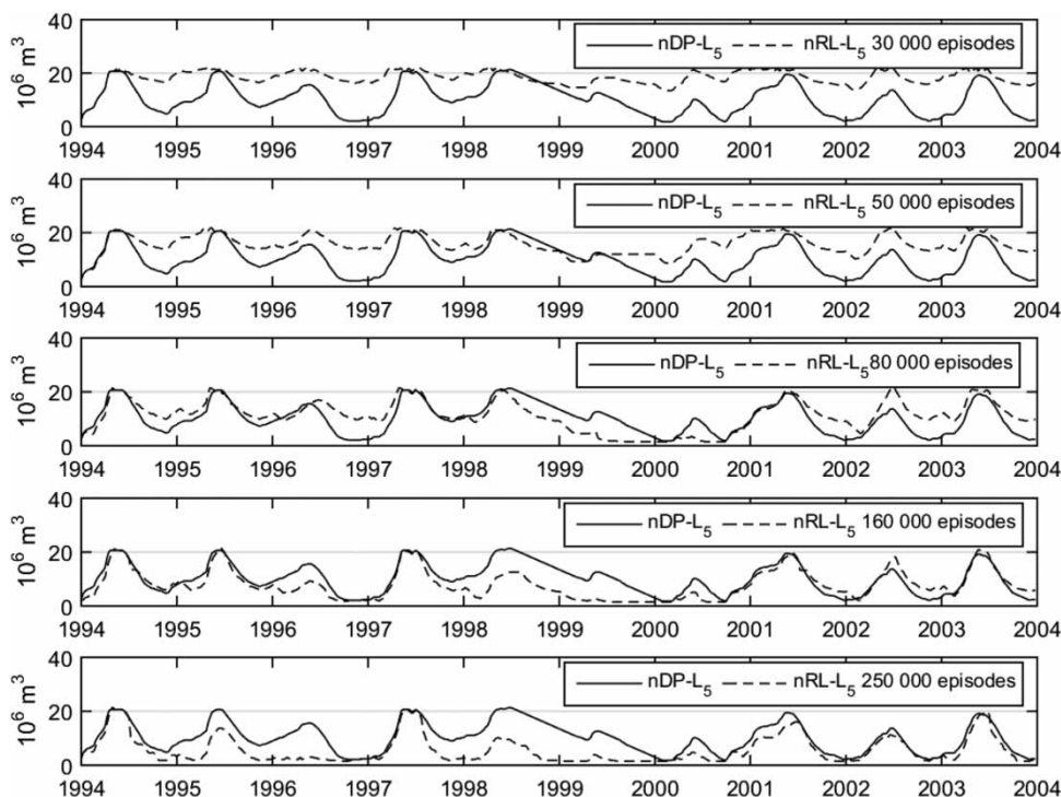
Figure 3 | nRL- L_5 agent learning with increasing the number of episodes: nDP- L_5 target reservoir storage (blue in online version) and nRL- L_5 obtained reservoir storage (red in online version) (testing period). Please refer to the online version of this paper to see this figure in colour: http://dx.doi.org/10.2166/hydro.2016.243 .
