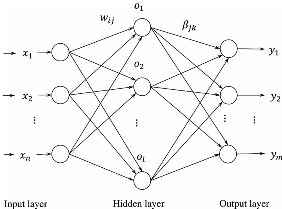
Figure 2 | Structure of the ELM.
