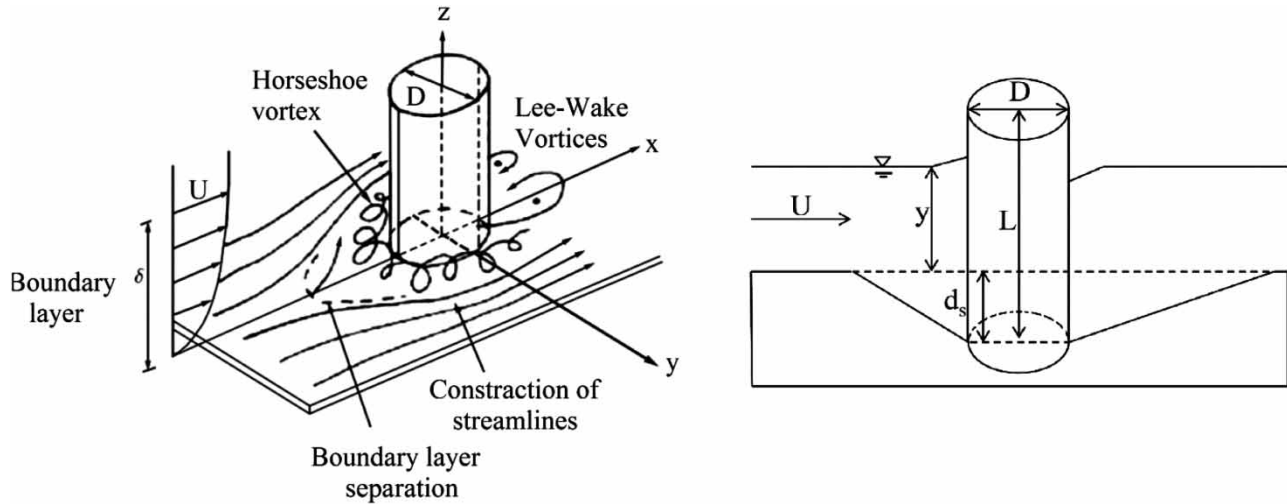
Figure 1 | Local scour and flow around cylindrical pier.
