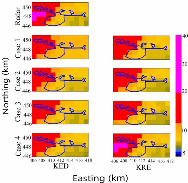
Figure 7 | Merged rainfall on 6 September 2008 for the KED merging method (left) and KRE method (right) and for the four cases of merging network. The top plot is the original radar data.
