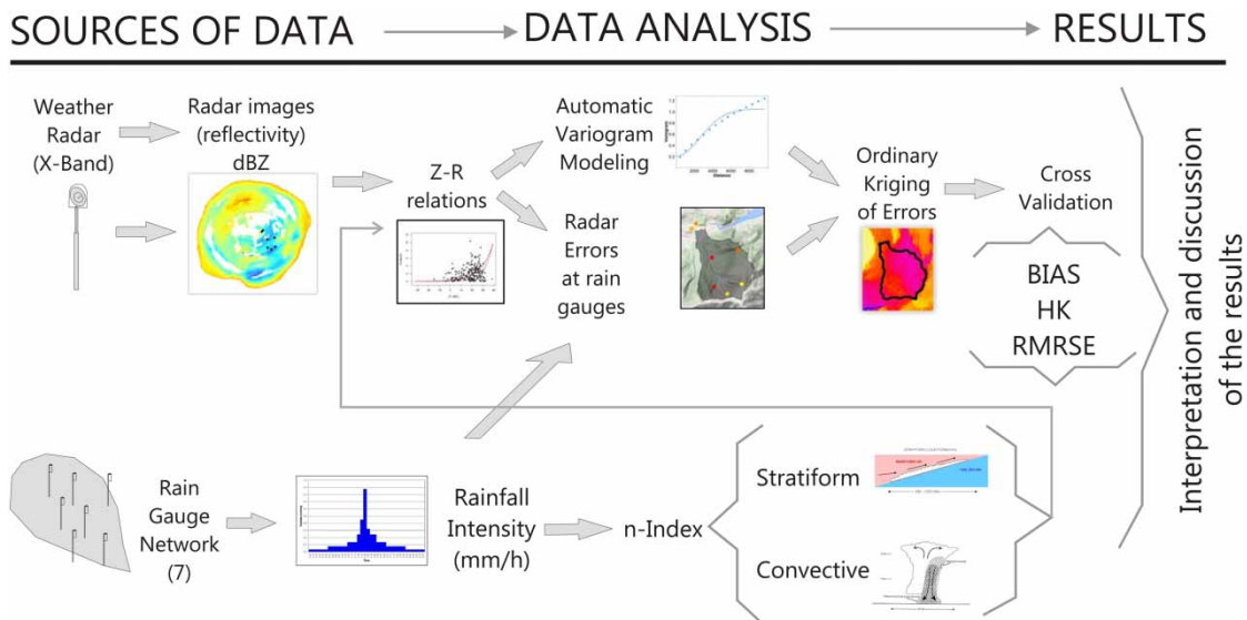
Figure 1 | Methodology scheme.
