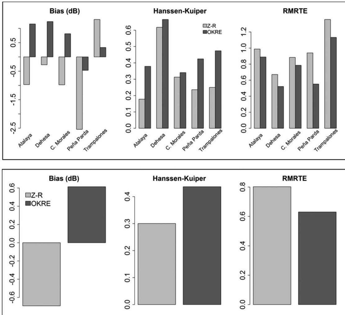
Figure 6 | Bias (dB), HK discriminant and RM RTE evaluated for all the available data (lower plot) and differentiating for the five rain gauges (upper plot).
