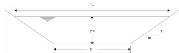
Figure 1 | A trapezoidal channel cross section.
