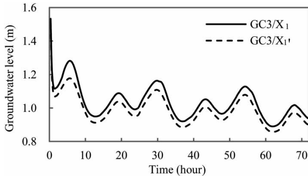
Figure 6 | Groundwater level fluctuations influenced by pumping in the landward and seaward locations.
