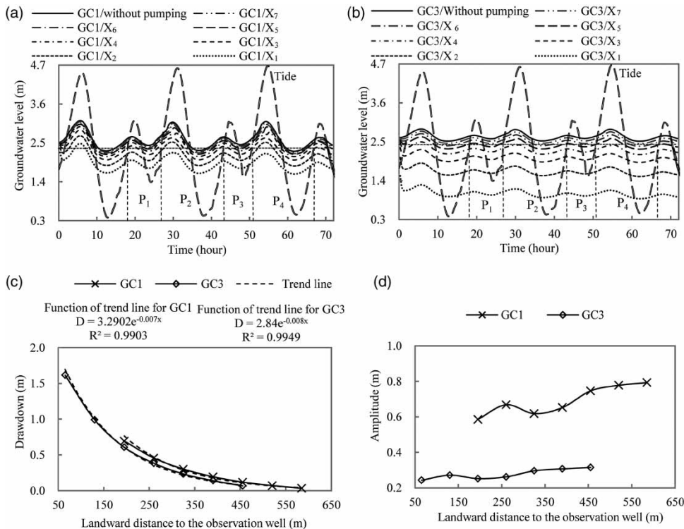
Figure 5 | Groundwater level dynamics in the observation wells with the pumping well located at different landward locations: (a) groundwater level fluctuation in GC1; (b) groundwater level fluctuation in GC3; (c) variation of the mean groundwater level drawdown, i.e., each trend line is defined by a function that expresses the relationship between the drawdown (represented by D in the function) and the landward distance (represented by x in the function); (d) variation of the amplitude.
