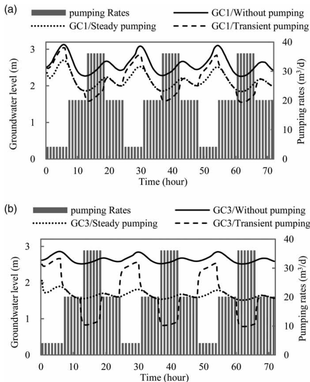
Figure 7 | Groundwater level fluctuations under transient pumping conditions: (a) GC1; (b) GC3.
