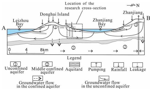
Figure 2 | Schematic cross-section of Donghai Island along the line AB in Figure 1(b) (cited from Zhou et al. (2014). Copyright: Springer-Verlag Berlin Heidelberg, 2013; Pengpeng Zhou).
