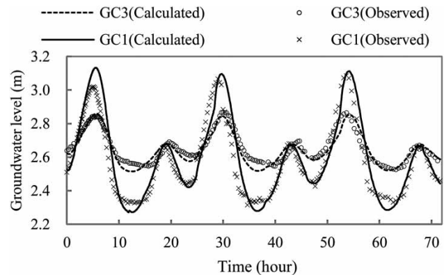
Figure 4 | Calibration map obtained for transient-state conditions.
