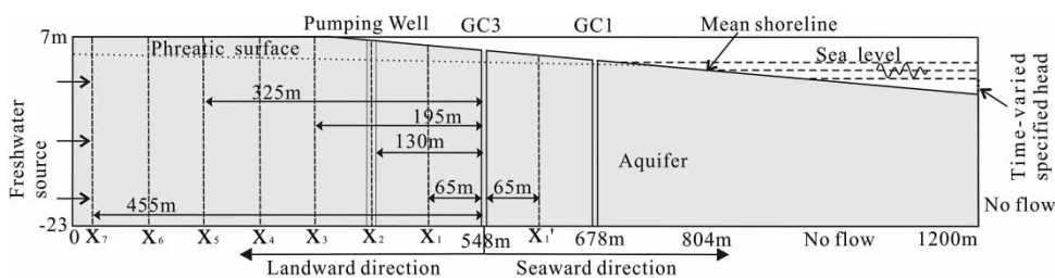
Figure 3 | Schematic of the conceptual model (revised from Zhou et al. (2014). Copyright: Springer-Verlag Berlin Heidelberg, 2013; Pengpeng Zhou).
