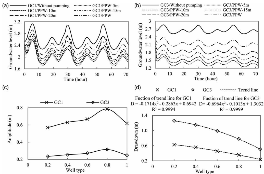
Figure 8 | Groundwater level dynamics in the observation wells with landward pumping in different types of partial penetration wells: (a) groundwater level fluctuation in GC1; (b) groundwater level fluctuation in GC3; (c) variation of the amplitude in the quasi-steady state; (d) variation of the mean groundwater level drawdown.
