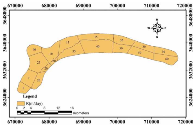
Figure 7 | Hydraulic conductivity polygons in Birjand aquifer.
